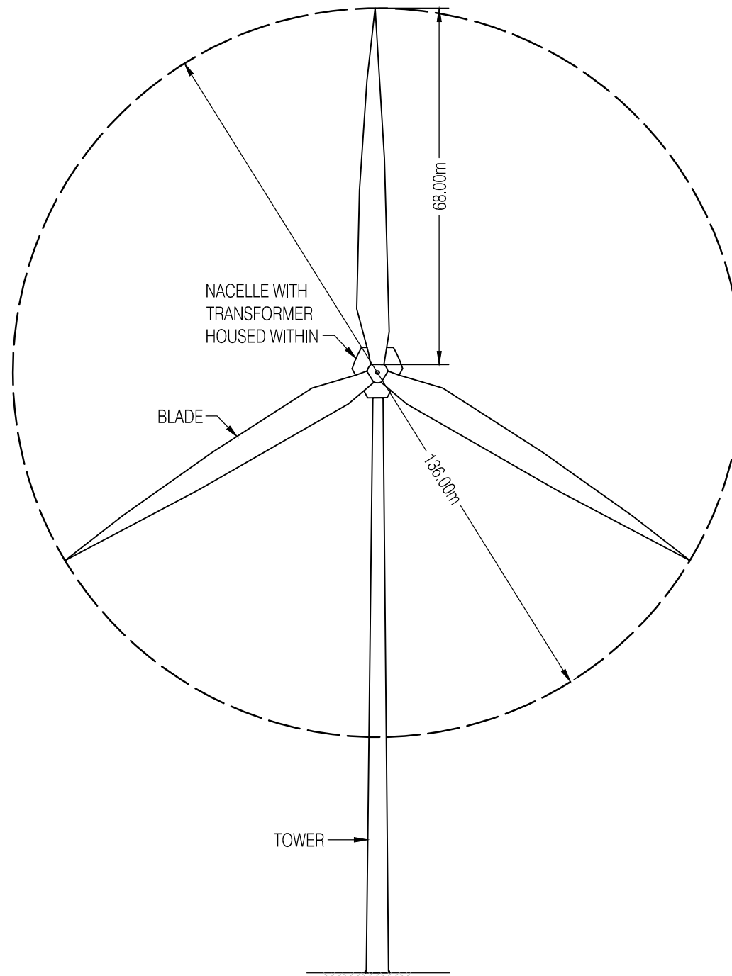
FRONT ELEVATION SCALE 1:1000
